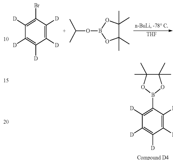
Compound D4
