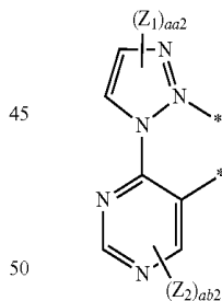
Formula 2-71
