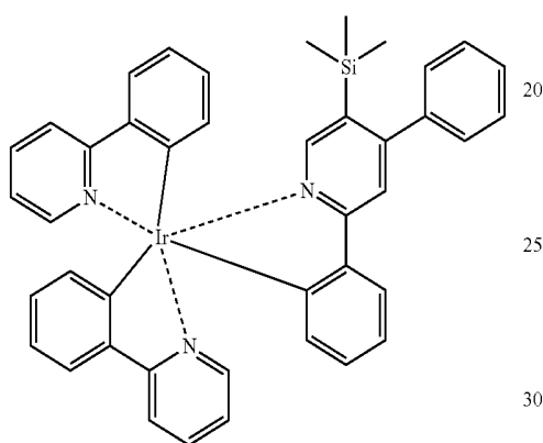
Compound 136
