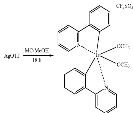
Compound M1A
