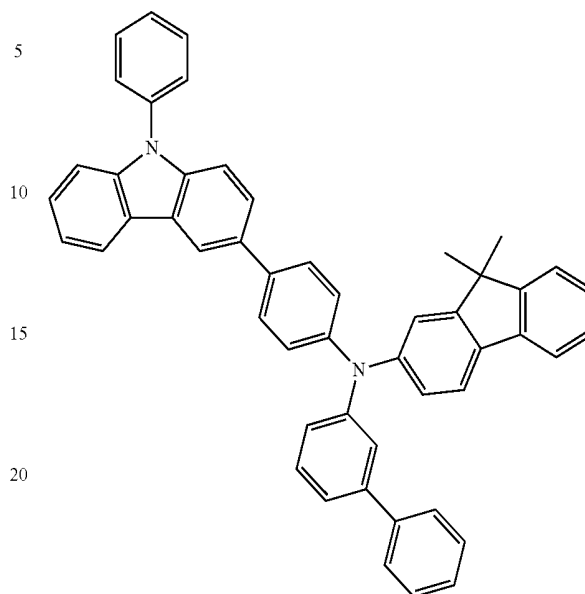
Formula 201A
