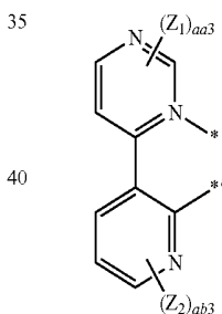
Formula 2-19
