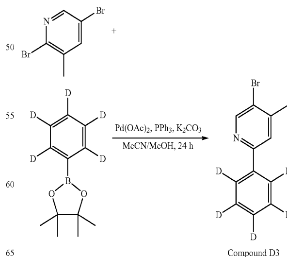
Compound D3
