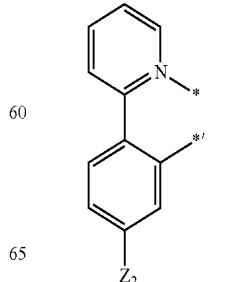
Formula 2-1(6)
