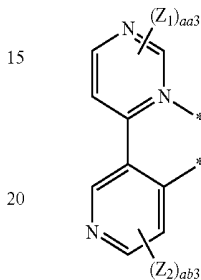
Formula 2-17
