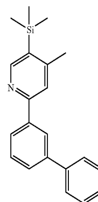
Compound B2
