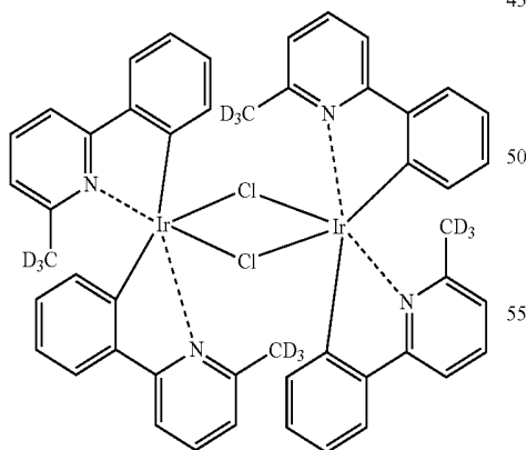
Compound M2C
