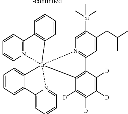
Compound 209
