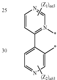
Formula 2-18
