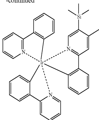
Comparative Compound 1
