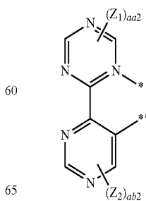
Formula 2-31
