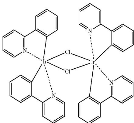
Compound M2A
