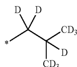
Formula 9-1 50
