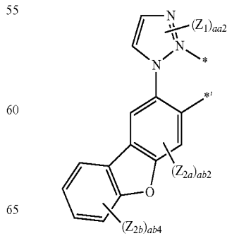
Formula 2-72
