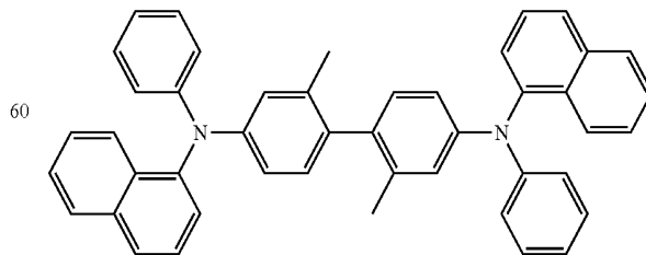
methylated NPB
