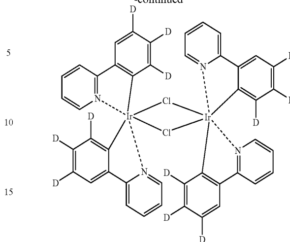
Compound M2B
