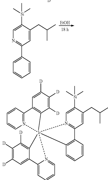
Compound 189
