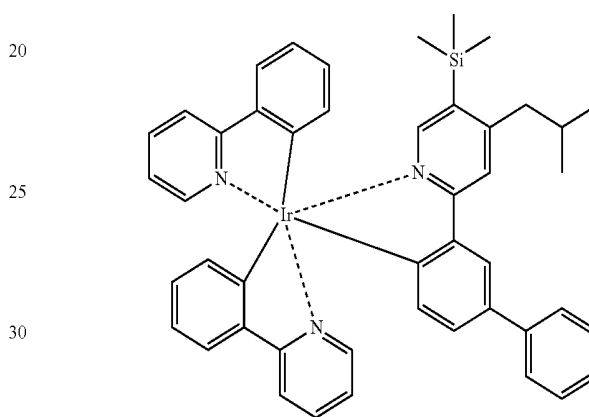
Compound 96
