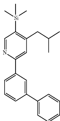
Compound B1
