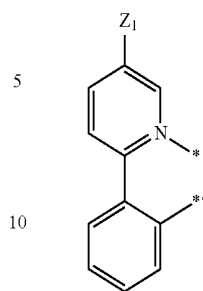
Formula 2-1(2)
