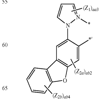
Formula 2-41
