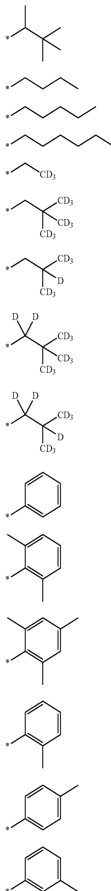
Formula 9-1
