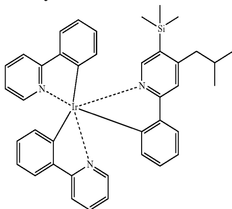
Compound 6
