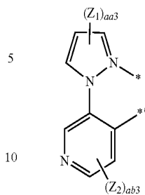
Formula 2-37
