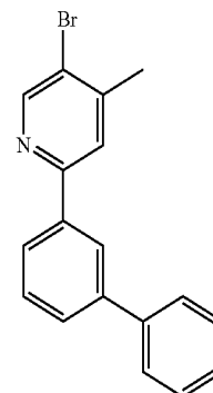
Compound B3
