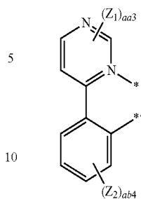
Formula 2-16
