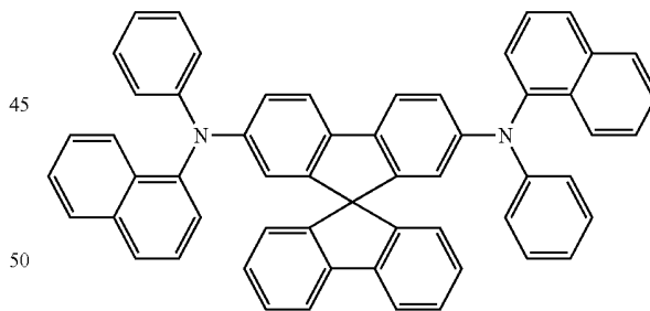
Spiro-NPB
