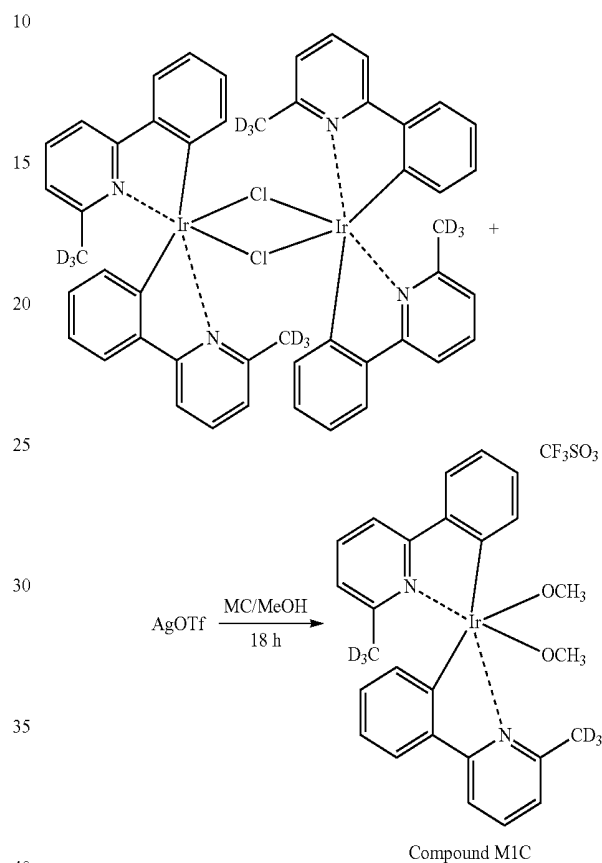
Compound M1C
