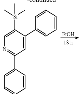
Compound C1
