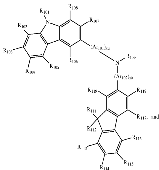
Formula 202
