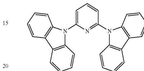
mCP
