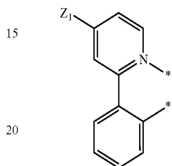
Formula 2-1(3)
