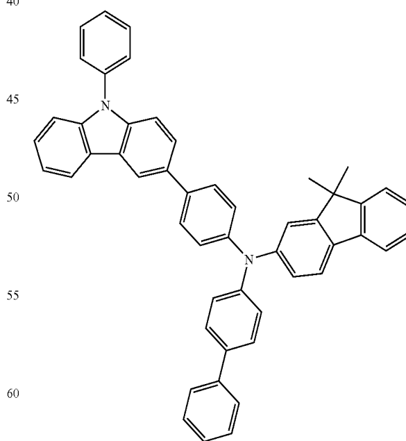
HT1
