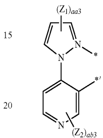
Formula 2-38
